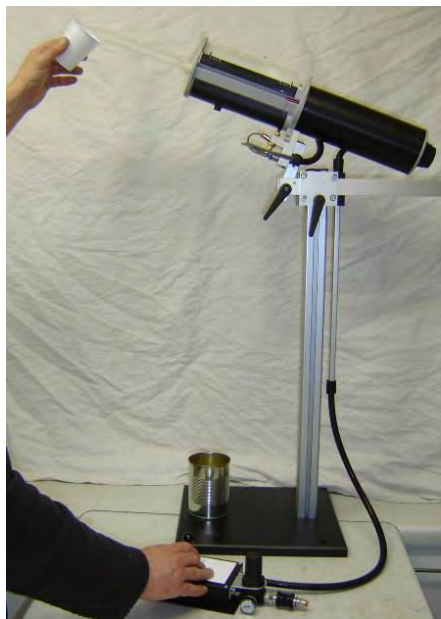
Multi axis adjustable gun support stand
